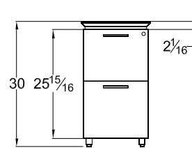
Pedestal Front Profile File/File
