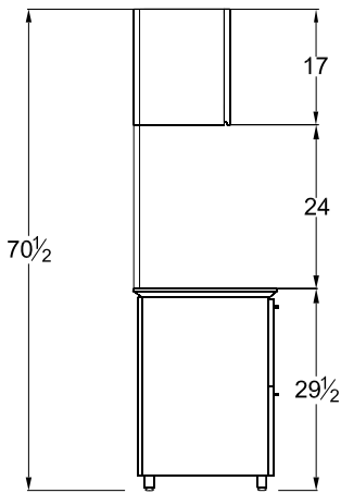
Typical Single Height Side Profile Wall Hung Overhead
