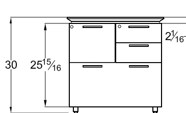
Pedestal Front Profile Multi-File
